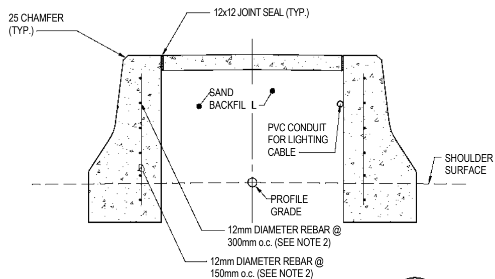
MEDIAN BARRIER TYPE "A" 1-25
